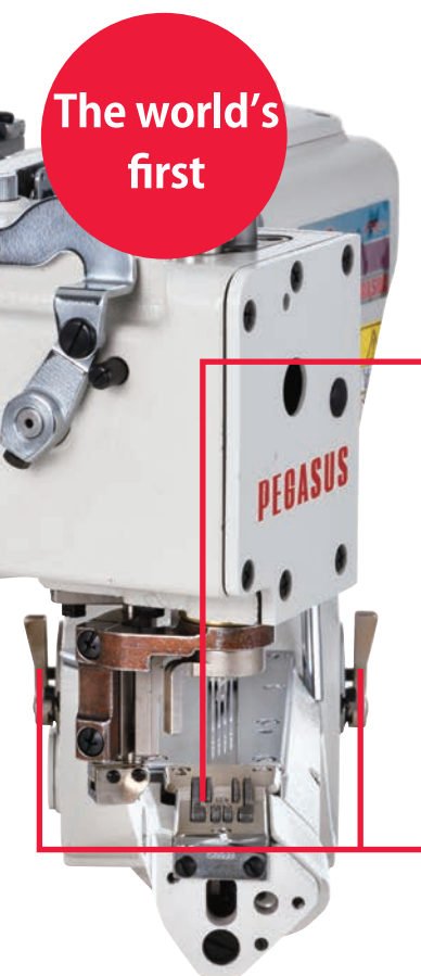
Right and left independent differential feed adjustment mechanism
